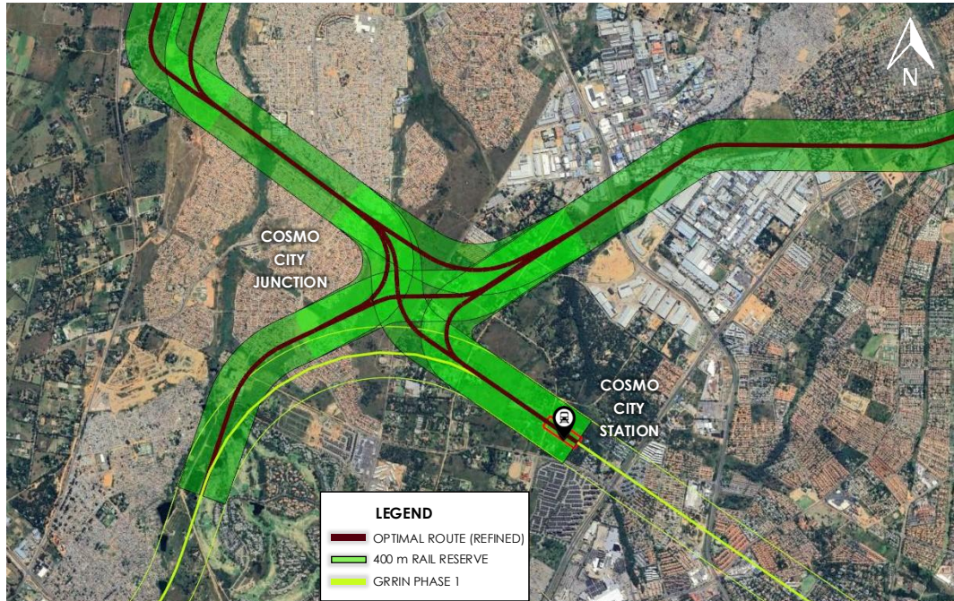
Figure 6-18: Cosmo City Junction and Rail Reserve Boundary
