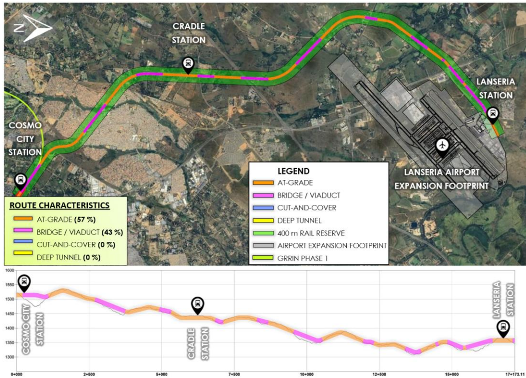
Figure 6-9: Option 1 – Cosmo City to Lanseria – Including Vertical Profile
